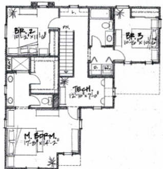
SECOND FLOOR SCALE: 1/8" = 1'-0"
